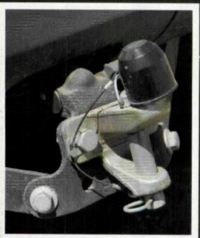
Tow ball/jaw unit: whether it's towing a heavy trailer or performing a vehicle recovery, this heavy-duty 3 500kg-rated unit is an essential piece of kit
